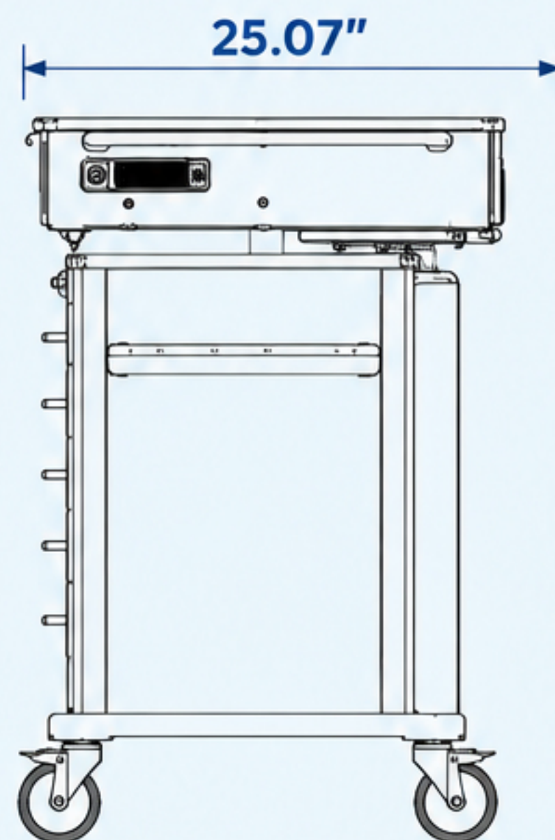
SIDE VIEW
